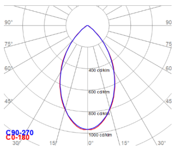
DRAGON 2.0 S-55_95W_4000K
