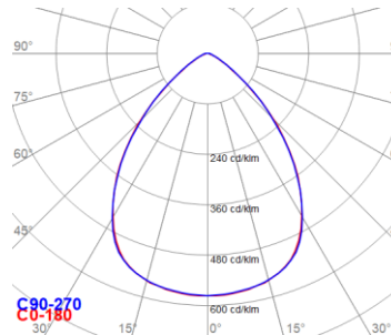
DRAGON 2.0 S-85_95W_4000K
