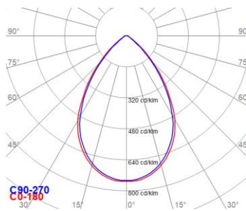
DRAGON 2.0 S-75_95W_4000K
