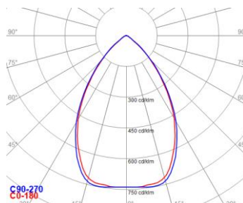
PETROL 2.0 NT-75_95W_4000K
